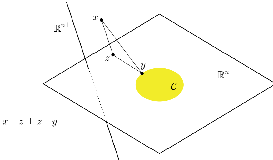
Figure 173: Closed convex set \mathcal{C} belongs to subspace \mathbb{R}^n (shown bounded in sketch and drawn without proper perspective). Point y is unique minimum-distance projection of x on \mathcal{C} ; equivalent to product of orthogonal projection of x on \mathbb{R}^n and minimum-distance projection of result z on \mathcal{C} .
