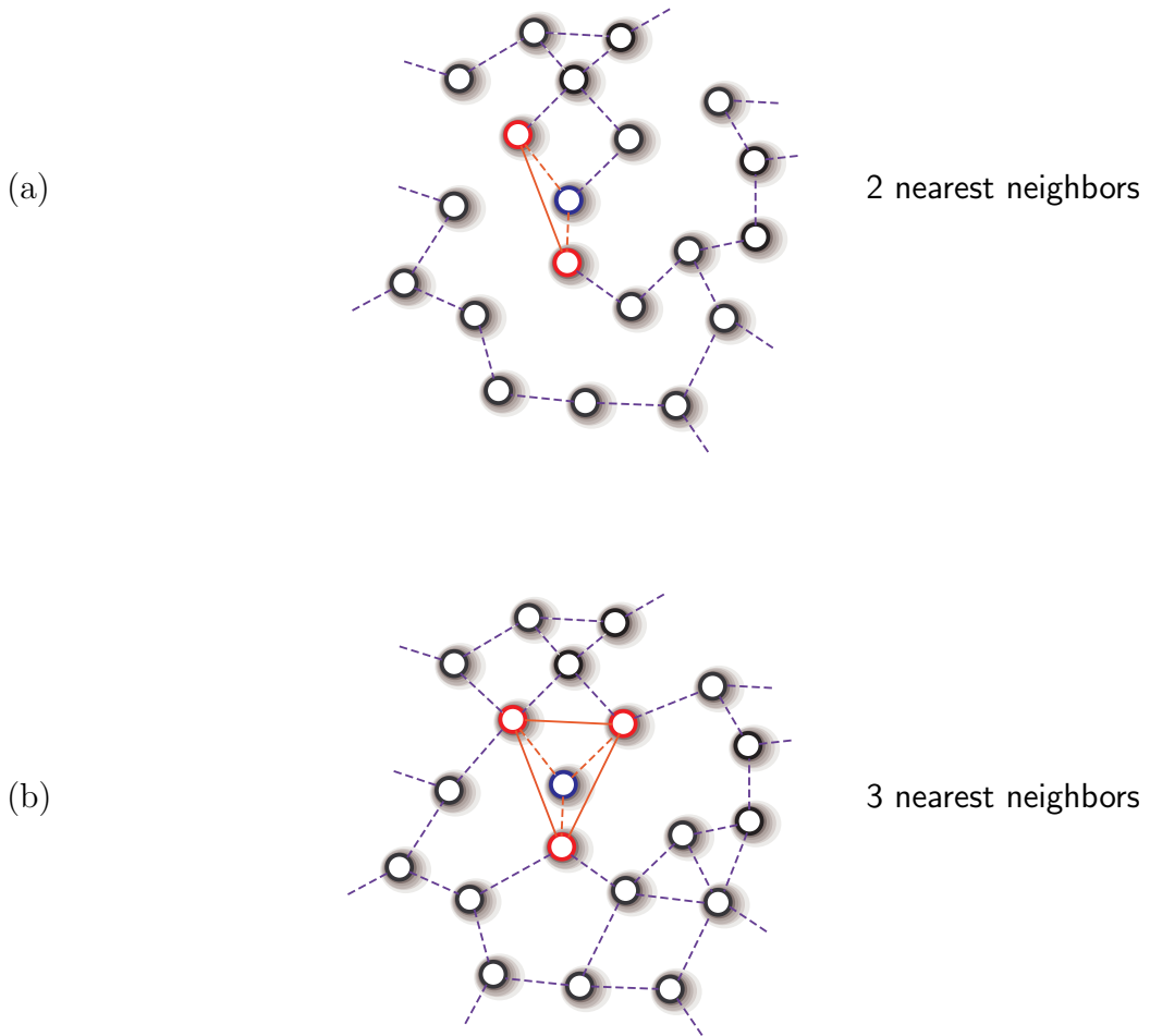
Figure 151: Neighborhood graph (dashed) with one dimensionless EDM subgraph completion (solid) superimposed (but not obscuring dashed). Local view of a few dense samples \circ from relative interior of some arbitrary Euclidean manifold whose affine dimension appears two-dimensional in this neighborhood. All line segments measure absolute distance. Dashed line segments help visually locate nearest neighbors; suggesting, best number of nearest neighbors can be greater than value of embedding dimension after topological transformation. ( confer [213, §2]) Solid line segments represent completion of EDM subgraph from available distance data for an arbitrarily chosen sample and its nearest neighbors. Each distance from EDM subgraph becomes distance-square in corresponding EDM submatrix.
