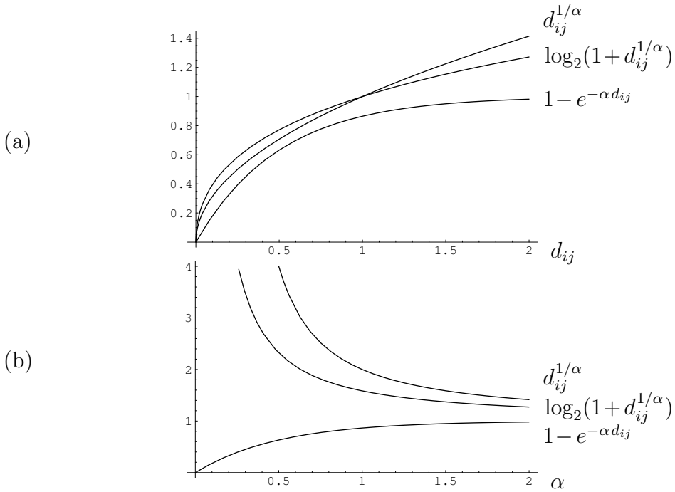
Figure 139: Some entrywise EDM compositions: (a) \alpha = 2 . Concave nondecreasing in d_{ij} . (b) Trajectory convergence in \alpha for d_{ij} = 2 .
