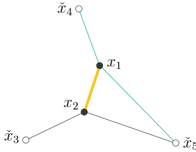
Figure 129: (Ye) Two sensors \bullet and three anchors \circ in \mathbb{R}^2 . Connecting line-segments denote known absolute distances. Incomplete EDM corresponding to this dimensionless EDM graph provides unique isometric reconstruction in \mathbb{R}^2 .
