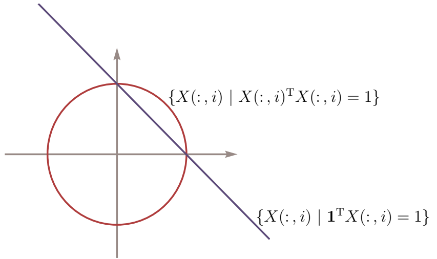
Figure 105: Permutation matrix i^{\text{th}} column-sum and column-norm constraint, abstract in two dimensions, when rank-1 constraint is satisfied. Optimal solutions reside at intersection of hyperplane with unit circle.
