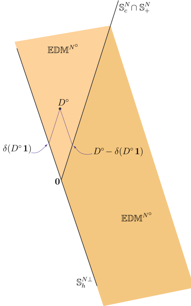
Figure 156: Hand-drawn abstraction of polar EDM cone (drawn truncated). Any member D^\circ of polar EDM cone can be decomposed into two linearly independent nonorthogonal components: \delta(D^\circ \mathbf{1}) and D^\circ - \delta(D^\circ \mathbf{1}) .
