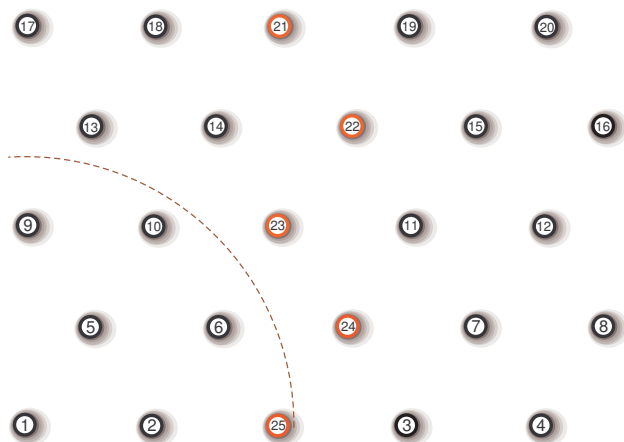
Figure 89: 5-lattice in \mathbb{R}^2 . Nodes 21 through 25 are anchors.
