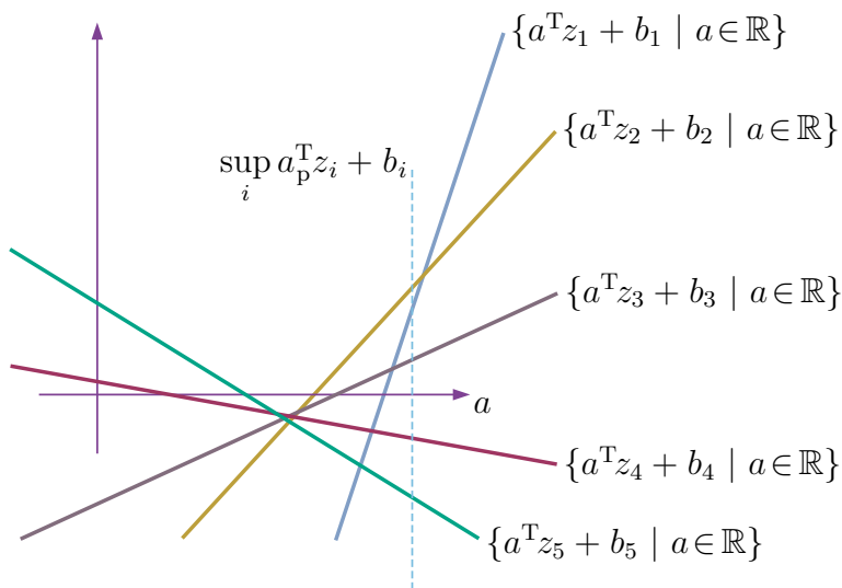
Figure 74: Pointwise supremum of any convex functions remains convex; by epigraph intersection. Supremum of affine functions in variable a evaluated at argument a_p is illustrated. Topmost affine function per a is supremum.
