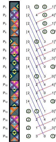
Figure 116: \bigcirc indicate boundary \beta , line segments indicate differences \Delta . Entries are indices \ell to standard basis vectors e_\ell \in \mathbb{R}^L from Figure 115.
