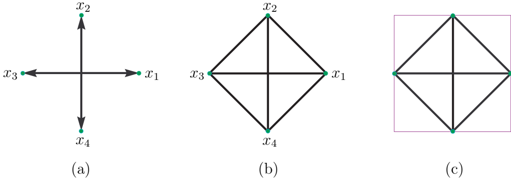
Figure 134: (a) Four points in quadrature in two dimensions about their geometric center. (b) Complete EDM graph of diamond-shaped vertices. (c) Quadrature rotation of a Euclidean body in \mathbb{R}^2 first requires a shroud that is the smallest Cartesian square containing it.
