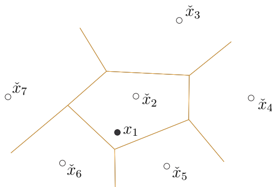
Figure 131: Regions of coverage by base stations \circ in a cellular telephone network. The term cellular arises from packing of regions best covered by neighboring base stations. Illustrated is a pentagonal cell best covered by base station \check{x}_2 . Like a Voronoi diagram, cell geometry depends on base-station arrangement. In some US urban environments, it is not unusual to find base stations spaced approximately 1 mile apart. There can be as many as 20 base-station antennae capable of receiving signal from any given cell phone \bullet ; practically, that number is closer to 6.
