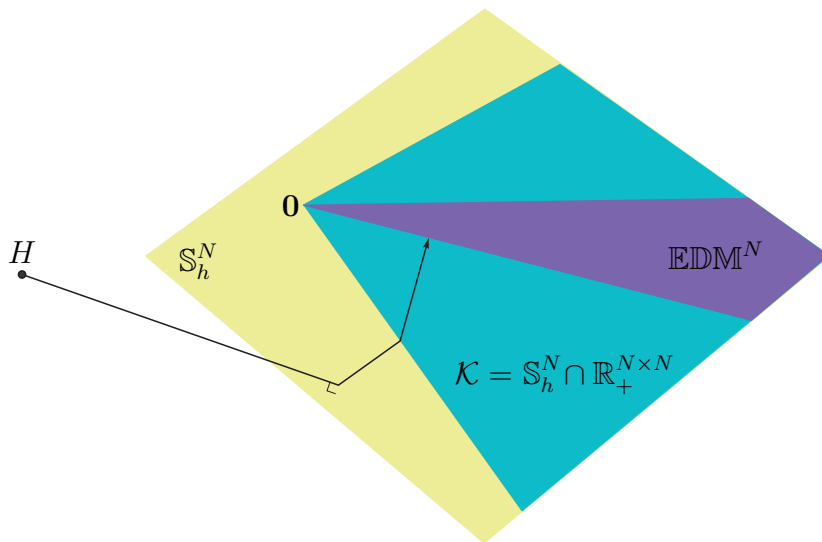
Figure 159: Pseudo-Venn diagram from Figure 158 showing elbow placed in path of projection of H on \text{EDM}^N \subset \mathbb{S}_h^N by an optimization problem demanding nonnegative input matrix H . The first two line segments leading away from H result from correct order-of-projection required to provide nonnegative H prior to optimization. Were H nonnegative, then its projection on \mathbb{S}_h^N would instead belong to \mathcal{K} ; making the elbow disappear. (confer Figure 173)
