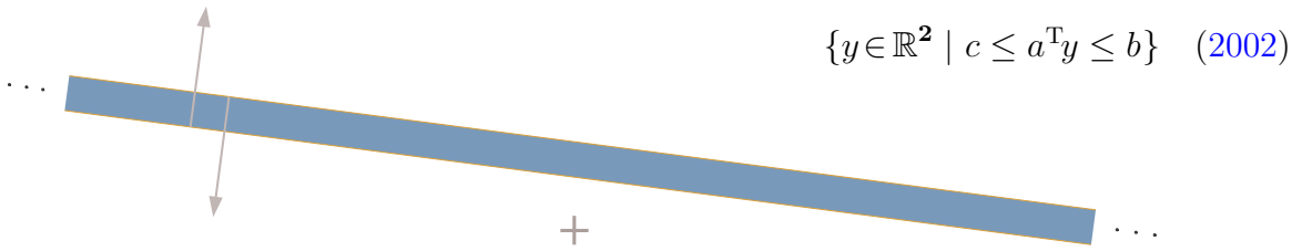
Figure 11: A slab is a convex Euclidean body infinite in extent but not affine. Illustrated in \mathbb{R}^2 , it may be constructed by intersecting two opposing halfspaces whose bounding hyperplanes are parallel but not coincident. Because number of halfspaces used in its construction is finite, slab is a polyhedron (§2.12). (Cartesian axes + and vector inward-normal, to each halfspace-boundary, are drawn for reference.)
