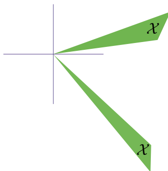
Figure 36: Union of two pointed closed convex cones is nonconvex cone \mathcal{X} .
