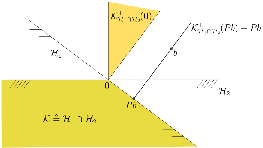
Figure 181: Two examples (truncated): normal cone to \mathcal{H}_1 \cap \mathcal{H}_2 at the origin and at point Pb on the boundary. \mathcal{H}_1 and \mathcal{H}_2 are the same halfspaces from Figure 180. Normal cone at the origin \mathcal{K}_{\mathcal{H}_1 \cap \mathcal{H}_2}^\perp(\mathbf{0}) is simply -\mathcal{K}^* .
