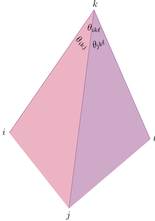
Figure 123: Fifth Euclidean metric property nomenclature. Each angle \theta is made by a vector pair at vertex k while i, j, k, \ell index four points at the vertices of a generally irregular tetrahedron. The fifth property is necessary for realization of four or more points; a reckoning by three angles in any dimension. Together with the first four Euclidean metric properties, this fifth property is necessary and sufficient for realization of four points.
