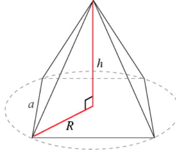
Figure 143: Length of one-dimensional face a equals height h=a=1 of this convex nonsimplicial pyramid in \mathbb{R}^3 with square base inscribed in a circle of radius R centered at the origin. [375, Pyramid ]
