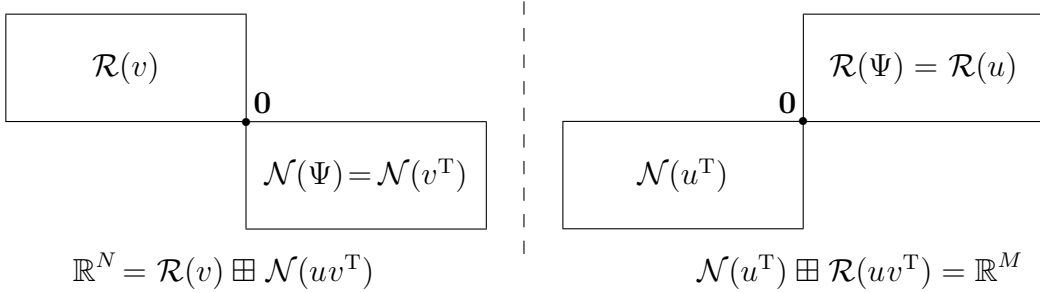
Figure 162: The four fundamental subspaces [334, §3.6] of any dyad \Psi = uv^T \in \mathbb{R}^{M \times N} : \mathcal{R}(v) \perp \mathcal{N}(\Psi) & \mathcal{N}(u^T) \perp \mathcal{R}(\Psi) . \Psi(x) \triangleq uv^T x is a linear mapping from \mathbb{R}^N to \mathbb{R}^M . Map from \mathcal{R}(v) to \mathcal{R}(u) is bijective. [332, §3.1]
