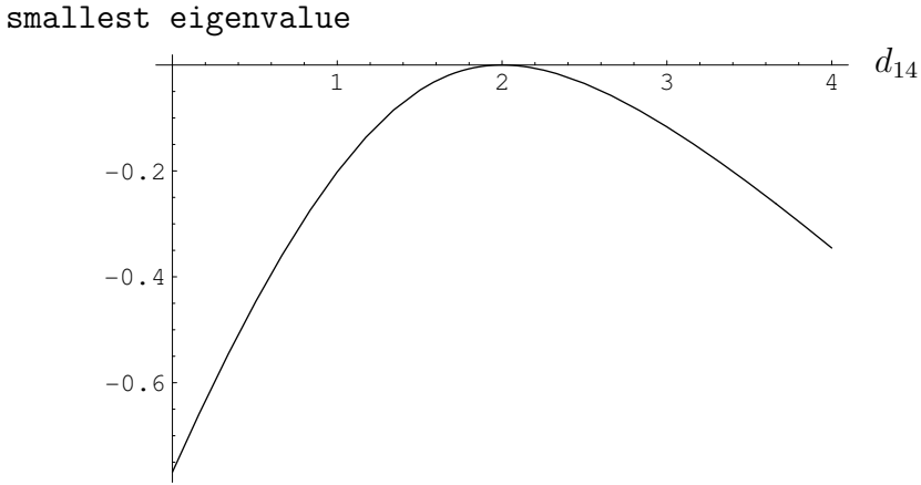
Figure 138: Smallest eigenvalue of -V_{\mathcal{N}}^T D V_{\mathcal{N}} makes it a PSD matrix for only one value of d_{14} : 2.
