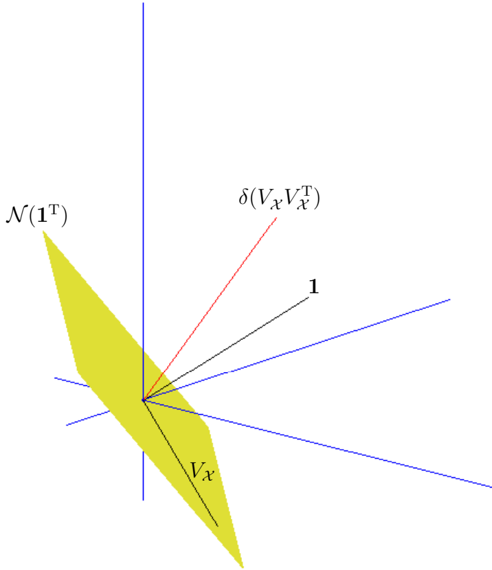
Figure 145: Example of V_{\mathcal{X}} selection to make an EDM corresponding to cardinality N=3 and affine dimension r=1 ; V_{\mathcal{X}} is a vector in nullspace \mathcal{N}(\mathbf{1}^T) \subset \mathbb{R}^3 . Nullspace of \mathbf{1}^T is hyperplane in \mathbb{R}^3 (drawn truncated) having normal \mathbf{1} . Vector \delta(V_{\mathcal{X}}V_{\mathcal{X}}^T) may or may not be in plane spanned by \{\mathbf{1}, V_{\mathcal{X}}\} , but belongs to nonnegative orthant which is strictly supported by \mathcal{N}(\mathbf{1}^T) .
