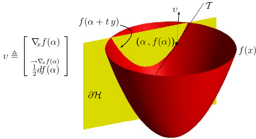
Figure 166: Strictly convex quadratic bowl in \mathbb{R}^2 \times \mathbb{R} ; f(x) = x^T x : \mathbb{R}^2 \rightarrow \mathbb{R} versus x on some open disc in \mathbb{R}^2 . Plane slice \partial\mathcal{H} is perpendicular to function domain. Slice intersection with domain connotes bidirectional vector y . Slope of tangent line \mathcal{T} at point (\alpha, f(\alpha)) is value of \nabla_x f(\alpha)^T y directional derivative (1874) at \alpha in slice direction y . Negative gradient -\nabla_x f(x) \in \mathbb{R}^2 is direction of steepest descent . [377] [220, §15.6] [153] When vector v \in \mathbb{R}^3 entry v_3 is half directional derivative in gradient direction at \alpha and when \begin{bmatrix} v_1 \\ v_2 \end{bmatrix} = \nabla_x f(\alpha) , then -v points directly toward bowl bottom.
