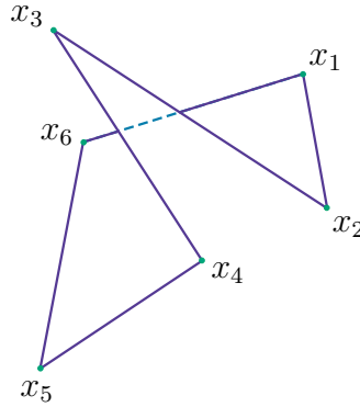
Figure 125: Arbitrary hexagon in \mathbb{R}^3 whose vertices are labelled clockwise.
