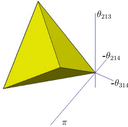
Figure 142: The relative-angle inequality tetrahedron (1196) bounding \mathbb{EDM}^4 is regular; drawn in entirety. Each angle \theta (987) must belong to this solid to be realizable.
