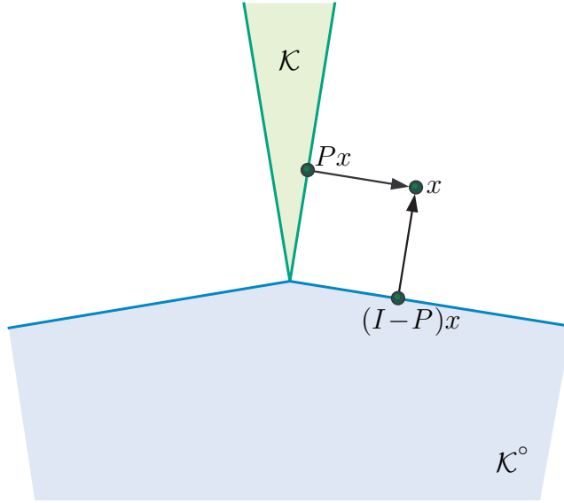
Figure 172: (confer Figure 171) Given minimum-distance projection (I-P)x of x on negative dual cone \mathcal{K}^\circ , projection on \mathcal{K} is immediate: x - (I-P)x = Px .
