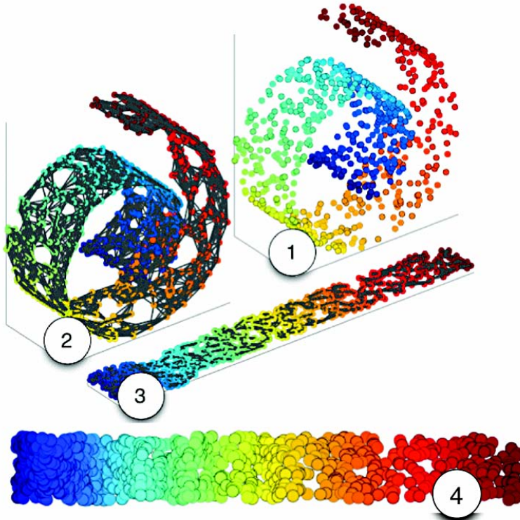
Figure 5: Swiss roll from Weinberger & Saul [374]. The problem of manifold learning, illustrated for N = 800 data points sampled from a “Swiss roll” ①. A discretized manifold is revealed by connecting each data point and its k=6 nearest neighbors ②. An unsupervised learning algorithm unfolds the Swiss roll while preserving the local geometry of nearby data points ③. Finally, the data points are projected onto the two dimensional subspace that maximizes their variance, yielding a faithful embedding of the original manifold ④.
