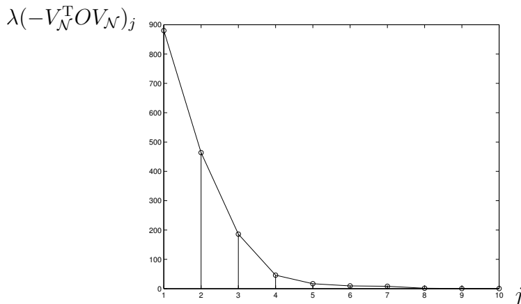
Figure 141: Largest ten eigenvalues, of -V_N^T O V_N for map of USA, sorted by nonincreasing value.
