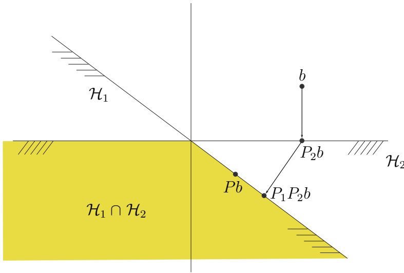
Figure 175: The sets \{\mathcal{C}_k\} in this example comprise two halfspaces \mathcal{H}_1 and \mathcal{H}_2 . The von Neumann-style alternating projection in \mathbb{R}^2 quickly converges to P_1P_2b (feasibility). Unique minimum-distance projection on the intersection is, of course, Pb .
