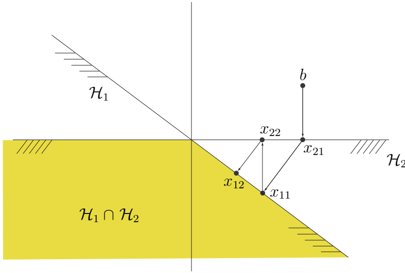
Figure 180: \mathcal{H}_1 and \mathcal{H}_2 are the same halfspaces as in Figure 175. Dykstra's alternating projection algorithm generates the alternations b, x_{21}, x_{11}, x_{22}, x_{12}, x_{12} \dots x_{12} . The path illustrated from b to x_{12} in \mathbb{R}^2 terminates at the desired result, Pb in Figure 175. The \{y_{ki}\} correspond to the first two difference vectors drawn (in the first iteration i=1 ), then oscillate between zero and a negative vector thereafter. These alternations are not so robust in presence of noise as for the example in Figure 174.
