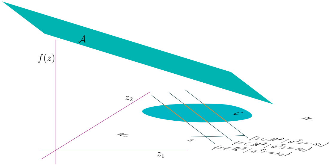
Figure 73: Three hyperplanes intersecting convex set \mathcal{C} \subset \mathbb{R}^2 from Figure 28. Cartesian axes in \mathbb{R}^3 : Plotted is affine subset \mathcal{A} = f(\mathbb{R}^2) \subset \mathbb{R}^2 \times \mathbb{R} ; a plane with third dimension. We say sequence of hyperplanes, w.r.t domain \mathbb{R}^2 of affine function f(z) = a^T z + b : \mathbb{R}^2 \rightarrow \mathbb{R} , is increasing in normal direction (Figure 26) because affine function increases in direction of gradient a (§3.6.0.0.3). Minimization of a^T z + b over \mathcal{C} is equivalent to minimization of a^T z .
