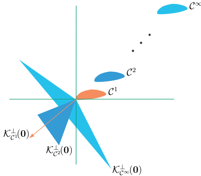
Figure 183: Rough sketch of normal cone to set \mathcal{C} \subset \mathbb{R}^2 as \mathcal{C} wanders toward infinity. A point at which a normal cone is determined, here the origin, need not belong to the set. Normal cone to \mathcal{C}^1 is a ray. But as \mathcal{C} moves outward, normal cone approaches a halfspace.
