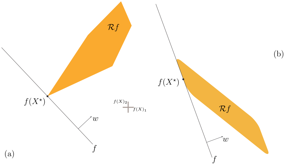
Figure 69: ( confer Figure 40) Function range is convex for a convex problem.
