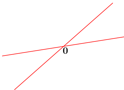
Figure 34: This nonconvex cone in \mathbb{R}^2 is a pair of lines through the origin. [251, §2.4] Because the lines are linearly independent, they are algebraic complements whose vector sum is \mathbb{R}^2 a convex cone.
