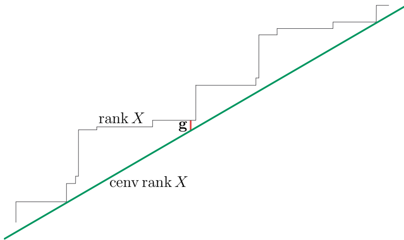
Figure 160: Abstraction of convex envelope of rank function. Rank is a quasiconcave function on positive semidefinite cone, but its convex envelope is the largest convex function whose epigraph contains it. Vertical bar labelled \mathbf{g} measures a trace/rank gap; id est , rank found always exceeds estimate; large decline in trace required here for only small decrease in rank.
