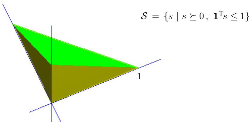
Figure 53: Unit simplex \mathcal{S} in \mathbb{R}^3 is a unique solid tetrahedron but not regular .
