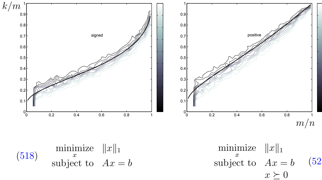
Figure 71: Exact recovery transition: Respectively signed [118] [120] or positive [125] [123] [124] solutions x to Ax=b with sparsity k below thick curve are recoverable. For Gaussian random matrix A \in \mathbb{R}^{m \times n} , thick curve demarcates phase transition in ability to find sparsest solution x by linear programming. These results were empirically reproduced in [38].
