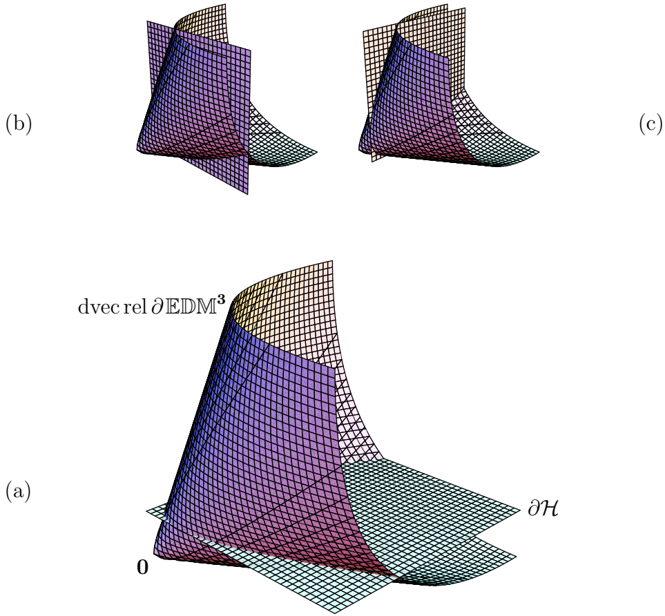
Figure 150: (a) In isometrically isomorphic subspace \mathbb{R}^3 , intersection of \text{EDM}^3 with hyperplane \partial\mathcal{H} representing one fixed symmetric entry d_{23} = \kappa (both drawn truncated, rounded vertex is artifact of plot). EDMs in this dimension corresponding to affine dimension 1 comprise relative boundary of EDM cone (§6.5). Since intersection illustrated includes a nontrivial subset of cone's relative boundary, then it is apparent there exist infinitely many EDM completions corresponding to affine dimension 1. In this dimension it is impossible to represent a unique nonzero completion corresponding to affine dimension 1, for example, using a single hyperplane because any hyperplane supporting relative boundary at a particular point \Gamma contains an entire ray \{\zeta\Gamma \mid \zeta \geq 0\} belonging to \text{rel } \partial\text{EDM}^3 by Lemma 2.8.0.0.1. (b) d_{13} = \kappa . (c) d_{12} = \kappa .
