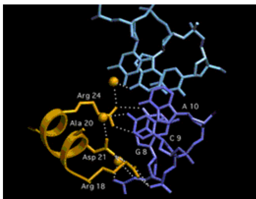
Figure 133: A depiction of molecular conformation . [117]
