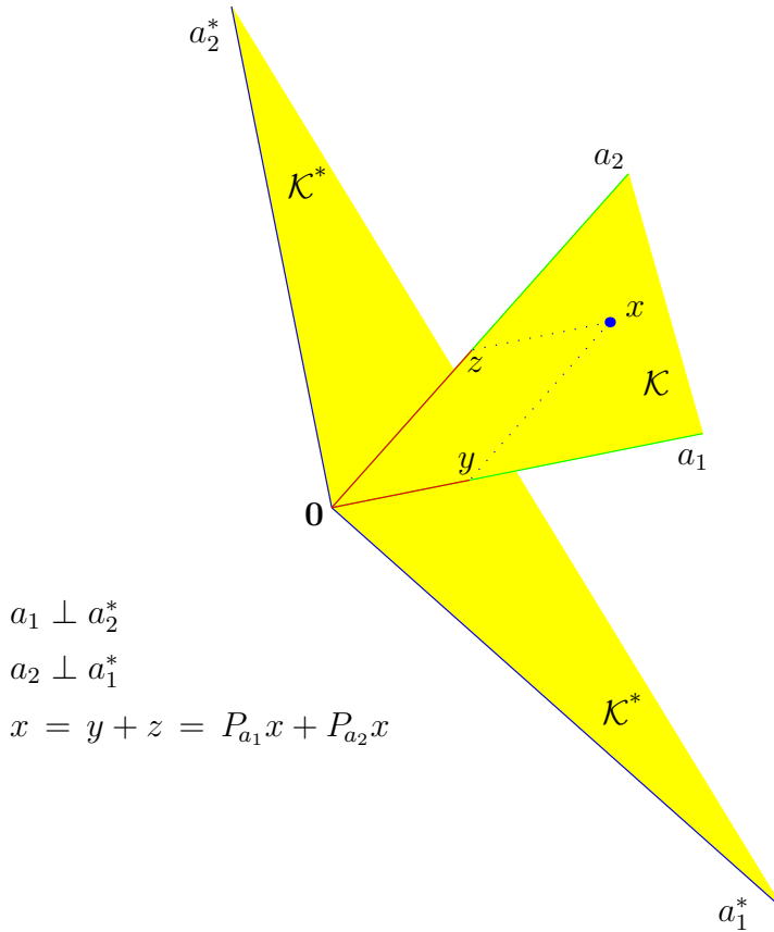
Figure 169: ( confer Figure 63) Biorthogonal expansion of point x \in \text{aff } \mathcal{K} is found by projecting x nonorthogonally on extreme directions of polyhedral cone \mathcal{K} \subset \mathbb{R}^2 . (Dotted lines of projection bound this translated negated cone.) Direction of projection P_{a_1} on extreme direction a_1 is orthogonal to extreme direction a_1^* of dual cone \mathcal{K}^* and parallel to a_2 (§E.3.5); similarly, direction of projection P_{a_2} on a_2 is orthogonal to a_2^* and parallel to a_1 . Point x is sum of nonorthogonal projections: x on \mathcal{R}(a_1) and x on \mathcal{R}(a_2) . Expansion is unique because extreme directions of \mathcal{K} are linearly independent. Were a_1 orthogonal to a_2 , then \mathcal{K} would be identical to \mathcal{K}^* and nonorthogonal projections would become orthogonal.
