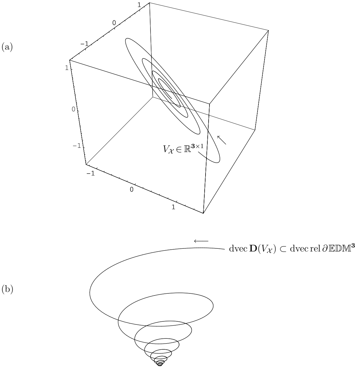
Figure 146: (a) Vector V_{\mathcal{X}} from Figure 145 spirals in \mathcal{N}(\mathbf{1}^T) \subset \mathbb{R}^3 decaying toward origin. (Spiral is two-dimensional in vector space \mathbb{R}^3 .) (b) Corresponding trajectory \mathbf{D}(V_{\mathcal{X}}) on EDM cone relative boundary creates a vortex also decaying toward origin. There are two complete orbits on EDM cone boundary about axis of revolution for every single revolution of V_{\mathcal{X}} about origin. (Vortex is three-dimensional in isometrically isomorphic \mathbb{R}^3 .)
