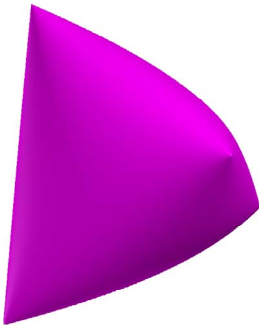
Figure 136: Elliptope \mathcal{E}^3 in isometrically isomorphic \mathbb{R}^6 (projected on \mathbb{R}^3 ) is a convex body that appears to possess some kind of symmetry in this dimension; it resembles a malformed pillow in the shape of a bulging tetrahedron. Elliptope relative boundary is not smooth and comprises all set members (1109) having at least one 0 eigenvalue. [239, §2.1] This elliptope has an infinity of vertices, but there are only four vertices corresponding to a rank-1 matrix. Those yy^T , evident in the illustration, have binary vector y \in \mathbb{R}^3 with entries in \{\pm 1\} .
