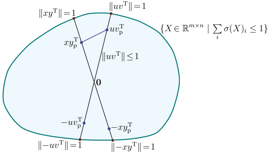
Figure 23: uv_p^T is a convex combination of normalized dyads \|\pm uv^T\|=1 ; similarly for xy_p^T . Any point in line segment joining xy_p^T to uv_p^T is expressible as a convex combination of two to four points indicated on boundary.
