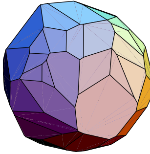
Figure 20: Convex hull of a random list of points in \mathbb{R}^3 . Some points from that generating list reside interior to this convex polyhedron (§2.12). [375, Convex Polyhedron ] (Avis-Fukuda-Mizukoshi)
