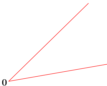
Figure 35: Boundary of a convex cone in \mathbb{R}^2 is a nonconvex cone; a pair of rays emanating from the origin.
