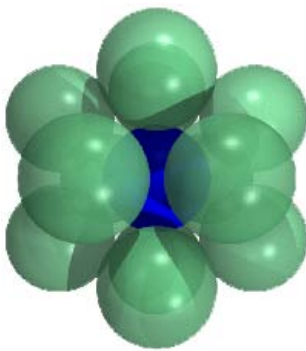
Figure 126: Sphere-packing illustration from [375, kissing number ]. Translucent balls illustrated all have the same diameter.
