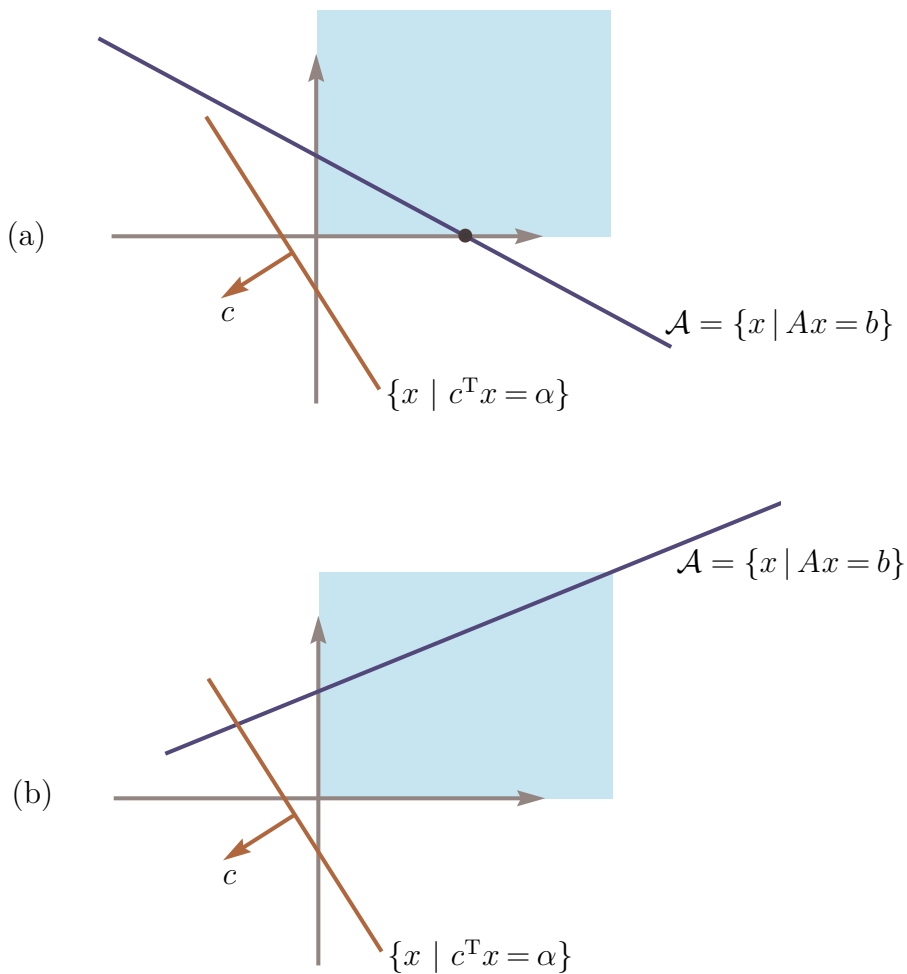
Figure 30: Minimizing hyperplane over affine set \mathcal{A} in nonnegative orthant \mathbb{R}^2_+ whose extreme directions (§2.8.1) are the nonnegative Cartesian axes. Solutions are visually ascertainable: (a) Optimal solution is \bullet . (b) Optimal objective \alpha^* = -\infty .
