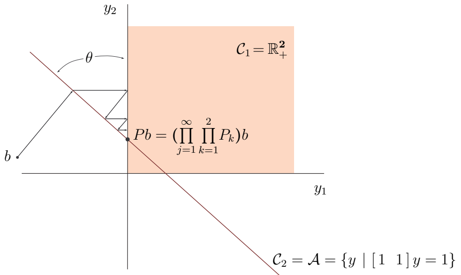
Figure 177: From Example E.10.2.0.2 in \mathbb{R}^2 , showing von Neumann-style alternating projection to find feasible solution belonging to intersection of nonnegative orthant with hyperplane \mathcal{A} . Point Pb lies at intersection of hyperplane with ordinate axis. In this particular example, feasible solution found is coincidentally optimal. Rate of convergence depends upon angle \theta ; as it becomes more acute, convergence slows. [176, §3]
