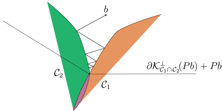
Figure 174: First several alternating projections in von Neumann-style projection (2103), of point b , converging on closest point Pb in intersection of two closed convex sets in \mathbb{R}^2 : C_1 and C_2 are partially drawn in vicinity of their intersection. Pointed normal cone \mathcal{K}^\perp (449) is translated to Pb , the unique minimum-distance projection of b on intersection. For this particular example, it is possible to start anywhere in a large neighborhood of b and still converge to Pb . Alternating projections are themselves robust with respect to significant noise because they belong to translated normal cone.
