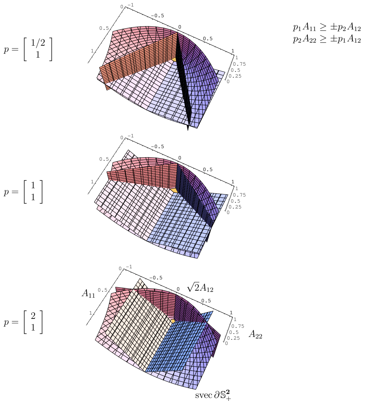
Figure 48: Proper polyhedral cone \mathcal{K} , created by intersection of halfspaces, inscribes PSD cone in isometrically isomorphic \mathbb{R}^3 as predicted by Geršgorin discs theorem for A = [A_{ij}] \in \mathbb{S}^2 . Hyperplanes supporting \mathcal{K} intersect along boundary of PSD cone. Four extreme directions of \mathcal{K} coincide with extreme directions of PSD cone.
