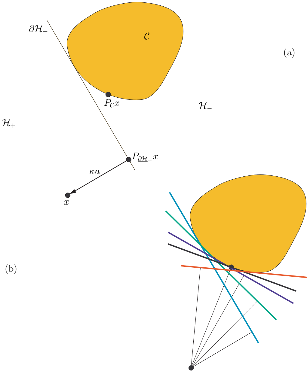
Figure 170: Dual interpretation of projection of point x on convex set \mathcal{C} in \mathbb{R}^2 . (a) \kappa = (a^T a)^{-1} (a^T x - \sigma_{\mathcal{C}}(a)) (b) Minimum distance from x to \mathcal{C} is found by maximizing distance to all hyperplanes supporting \mathcal{C} and separating it from x . A convex problem for any convex set, distance of maximization is unique.
