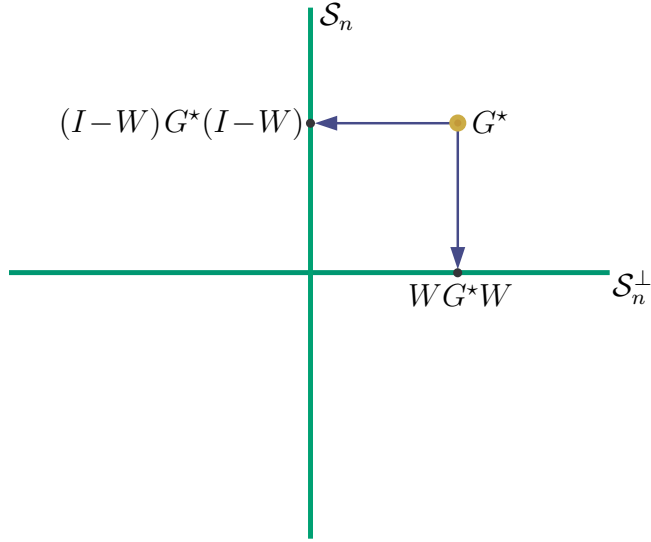
Figure 83: ( confer Figure 171) Projection of G^* on subspace \mathcal{S}_n of rank \leq n matrices whose nullspace contains \mathcal{N}(G^*) . This direction W is closed-form solution to (1739a).
