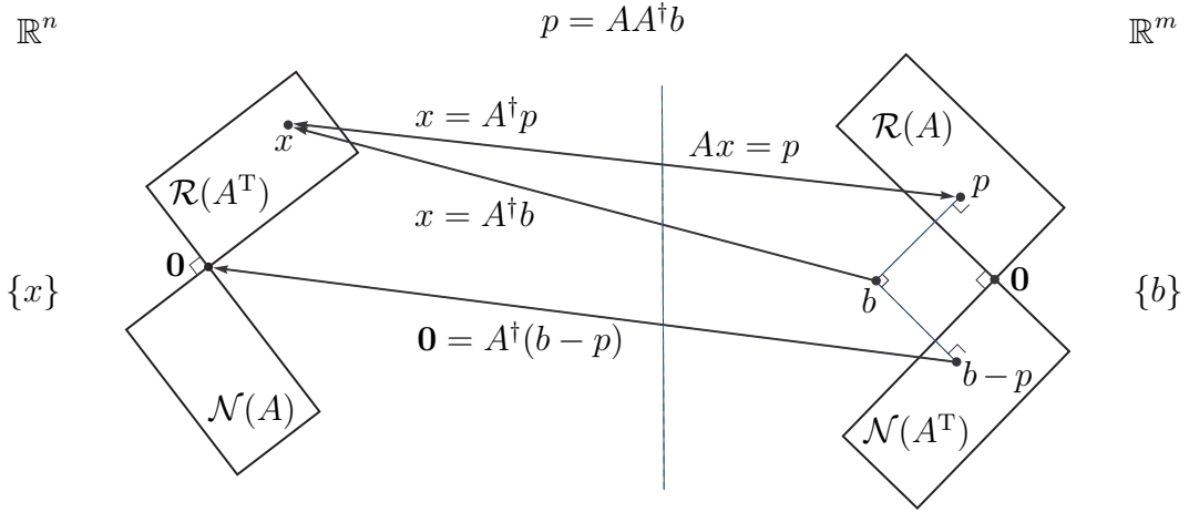
Figure 167: (confer Figure 16) Pseudoinverse A^\dagger \in \mathbb{R}^{n \times m} action: [332, p.449] Component of b in \mathcal{N}(A^T) maps to \mathbf{0} , while component of b in \mathcal{R}(A) maps to rowspace \mathcal{R}(A^T) . For any A \in \mathbb{R}^{m \times n} , inversion is bijective \forall p \in \mathcal{R}(A) . x = A^\dagger b \Leftrightarrow x \in \mathcal{R}(A^T) \ \& \ b - Ax \perp \mathcal{R}(A) \Leftrightarrow x \perp \mathcal{N}(A) \ \& \ b - Ax \in \mathcal{N}(A^T) . [48]
