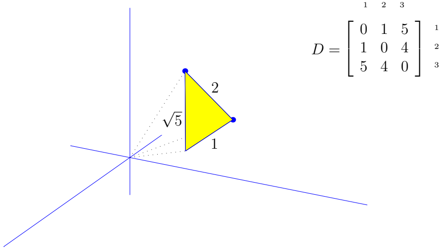
Figure 121: Convex hull of three points ( N=3 ) is shaded in \mathbb{R}^3 ( n=3 ). Dotted lines are imagined vectors to points whose affine dimension is 2.
