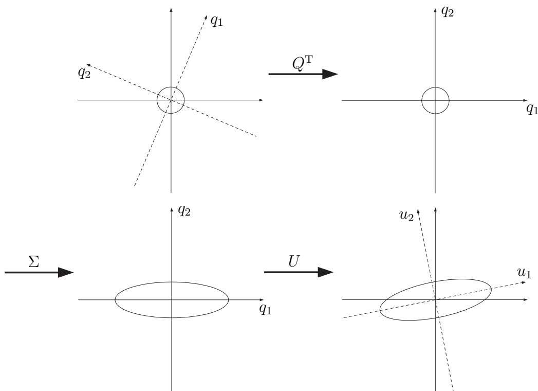
Figure 161: Geometrical interpretation of full SVD [272]: Image of circle \{x \in \mathbb{R}^2 \mid \|x\|_2 = 1\} under matrix multiplication Ax is, in general, an ellipse. For the example illustrated, U \triangleq [u_1 \ u_2] \in \mathbb{R}^{2 \times 2} , Q \triangleq [q_1 \ q_2] \in \mathbb{R}^{2 \times 2} .
