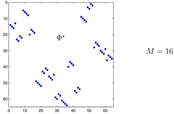
Figure 117: Sparsity pattern for composite permutation matrix \Phi^* \in \mathbb{R}^{4M \times 4M} representing solution from Figure 112b. Each four-point cluster represents a circulant permutation matrix from (867). Any M=16 -piece solution may be verified on the TOMY website .
