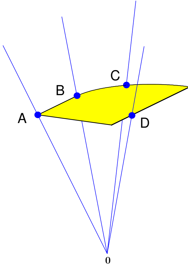
Figure 42: Properties of extreme points carry over to extreme directions. [308, §18] Four rays (drawn truncated) on boundary of conic hull of two-dimensional closed convex set from Figure 32 lifted to \mathbb{R}^3 . Ray through point A is exposed hence extreme. Extreme direction B on cone boundary is not an exposed direction, although it belongs to the exposed face \text{cone}\{A, B\} . Extreme ray through C is exposed. Point D is neither an exposed or extreme direction although it belongs to a two-dimensional exposed face of the conic hull.
