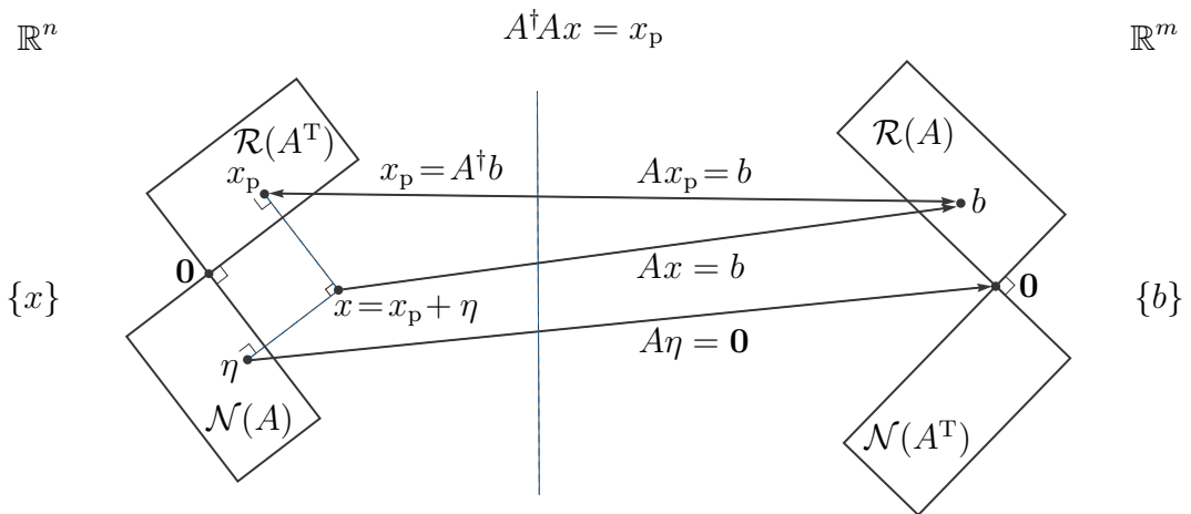
Figure 16: (confer Figure 167) Action of linear map represented by A \in \mathbb{R}^{m \times n} : Component of vector x in nullspace \mathcal{N}(A) maps to origin while component in rowspace \mathcal{R}(A^T) maps to range \mathcal{R}(A) . For any A \in \mathbb{R}^{m \times n} , AA^\dagger Ax = b (§E) and inverse image of b \in \mathcal{R}(A) is a nonempty affine set: x_p + \mathcal{N}(A) .
