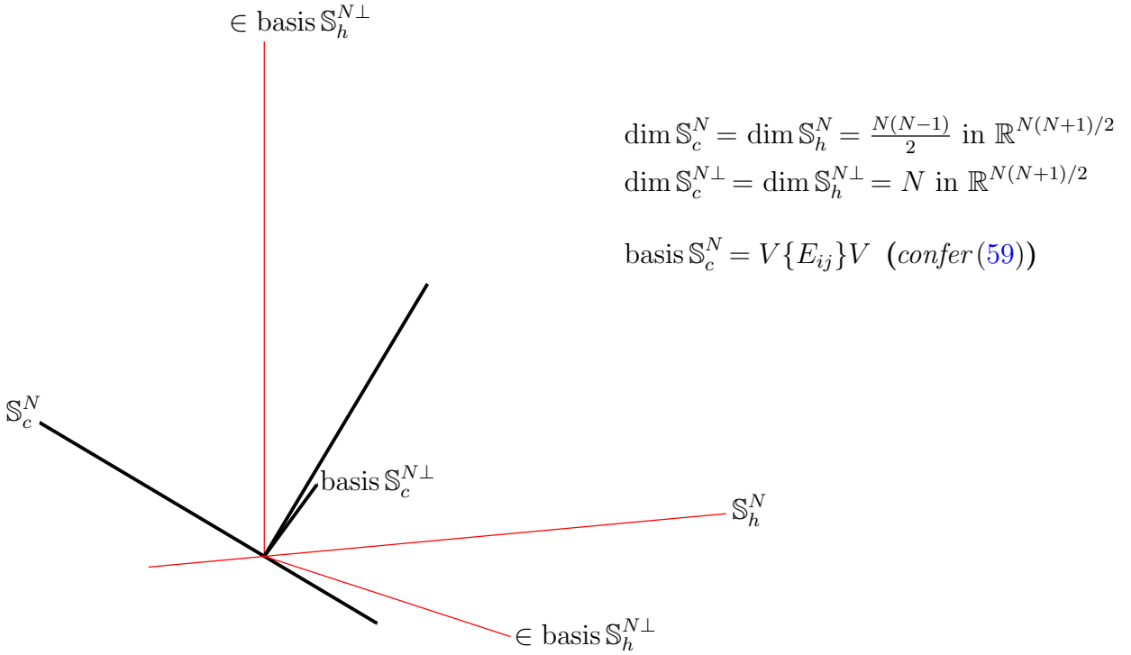
Figure 135: Orthogonal complements in \mathbb{S}^N abstractly oriented in isometrically isomorphic \mathbb{R}^{N(N+1)/2} . Case N=2 accurately illustrated in \mathbb{R}^3 . Orthogonal projection of basis for \mathbb{S}_h^{N\perp} on \mathbb{S}_c^{N\perp} yields another basis for \mathbb{S}_c^{N\perp} . (Basis vectors for \mathbb{S}_c^{N\perp} are illustrated lying in a plane orthogonal to \mathbb{S}_c^N in this dimension. Basis vectors for each \perp space outnumber those for its respective orthogonal complement; such is not the case in higher dimension.)
