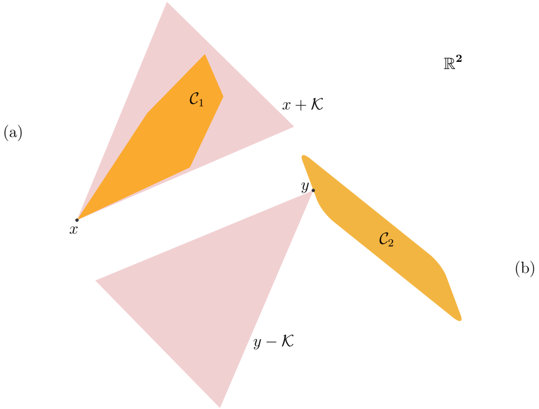
Figure 40: ( confer Figure 69) (a) Point x is the minimum element of set \mathcal{C}_1 with respect to cone \mathcal{K} because cone translated to x \in \mathcal{C}_1 contains entire set. (Cones drawn truncated.) (b) Point y is a minimal element of set \mathcal{C}_2 with respect to cone \mathcal{K} because negative cone translated to y \in \mathcal{C}_2 contains only y . These concepts, minimum/minimal, become equivalent under a total order .
