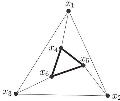
Figure 128: Incomplete EDM corresponding to this dimensionless EDM graph provides unique isometric reconstruction in \mathbb{R}^2 . (drawn freehand; no symmetry intended, confer (976))
