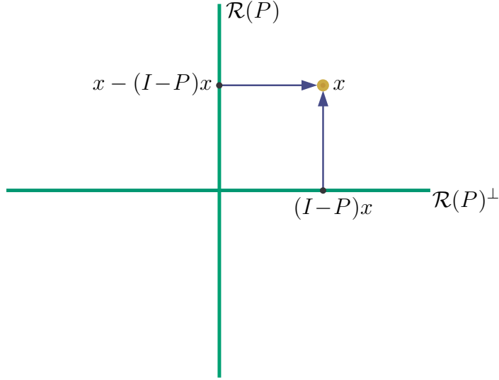
Figure 171: ( confer Figure 83, Figure 172) Given orthogonal projection (I - P)x of x on orthogonal complement \mathcal{R}(P)^\perp , projection on \mathcal{R}(P) is immediate: x - (I - P)x .
