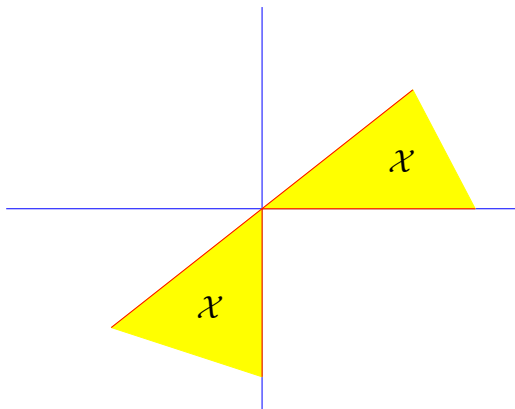
Figure 37: Truncated nonconvex cone \mathcal{X} = \{x \in \mathbb{R}^2 \mid x_1 \geq x_2, x_1 x_2 \geq 0\} . Boundary is also a cone. [251, §2.4] Cartesian axes drawn for reference. Each half (about the origin) is itself a convex cone.
