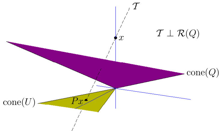
Figure 168: Nonorthogonal projection of x \in \mathbb{R}^3 on \mathcal{R}(U) = \mathbb{R}^2 under biorthogonality condition; id est , Px = UQ^T x such that Q^T U = I . Any point along imaginary line \mathcal{T} connecting x to Px will be projected nonorthogonally on Px with respect to horizontal plane constituting \mathbb{R}^2 = \text{aff cone}(U) in this example. Extreme directions of \text{cone}(U) correspond to two columns of U ; likewise for \text{cone}(Q) . For purpose of illustration, we truncate each conic hull by truncating coefficients of conic combination at unity. Conic hull \text{cone}(Q) is headed upward at an angle, out of plane of page. Nonorthogonal projection would fail were \mathcal{N}(Q^T) in \mathcal{R}(U) (were \mathcal{T} parallel to a line in \mathcal{R}(U) ).
