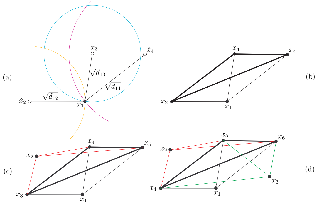
Figure 127: (a) Given three distances indicated with absolute point positions \check{x}_2, \check{x}_3, \check{x}_4 known and noncollinear, absolute position of x_1 in \mathbb{R}^2 can be precisely and uniquely determined by trilateration ; solution to a system of nonlinear equations. Dimensionless EDM graphs (b) (c) (d) represent EDMs in various states of completion. Line segments represent known absolute distances and may cross without vertex at intersection. (b) Four-point list must always be embeddable in affine subset having dimension \text{rank } V_N^T D V_N not exceeding 3. To determine relative position of x_2, x_3, x_4 , triangle inequality is necessary and sufficient (§5.14.1). Knowing all distance information, then (by injectivity of \mathbf{D} (§5.6)) point position x_1 is uniquely determined to within an isometry in any dimension. (c) When fifth point is introduced, only distances to x_3, x_4, x_5 are required to determine relative position of x_2 in \mathbb{R}^2 . Graph represents first instance of missing distance information; \sqrt{d_{12}} . (d) Three distances are absent ( \sqrt{d_{12}}, \sqrt{d_{13}}, \sqrt{d_{23}} ) from complete set of interpoint distances, yet unique isometric reconstruction (§5.4.2.3.7) of six points in \mathbb{R}^2 is certain.
