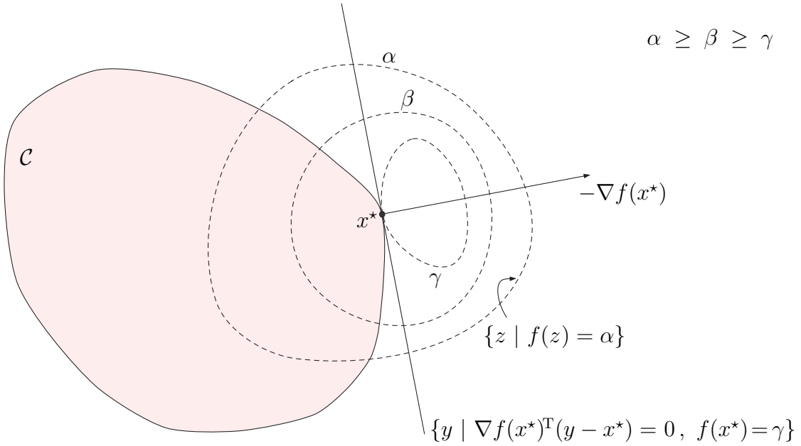
Figure 67: ( confer Figure 78) Shown is a plausible contour plot in \mathbb{R}^2 of some arbitrary differentiable convex real function f(x) at selected levels \alpha , \beta , and \gamma ; id est , contours of equal level f ( level sets ) drawn dashed in function's domain. From results in §3.6.2 (p.256), gradient \nabla f(x^*) is normal to \gamma -sublevel set \mathcal{L}_\gamma f (559) by Definition E.9.1.0.1. From §2.13.10.1, function is minimized over convex set \mathcal{C} at point x^* iff negative gradient -\nabla f(x^*) belongs to normal cone to \mathcal{C} there. In circumstance depicted, normal cone is a ray whose direction is coincident with negative gradient. So, gradient is normal to a hyperplane supporting both \mathcal{C} and the \gamma -sublevel set.
