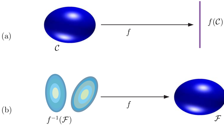
Figure 15: (a) Image of convex set in domain of any convex function f is convex, but there is no converse. (b) Inverse image under convex function f .
