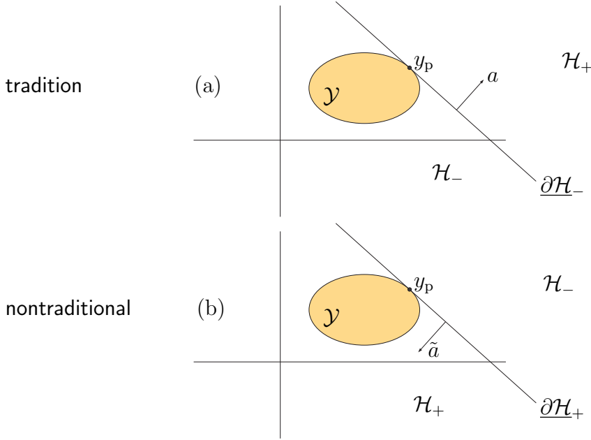
Figure 29: (a) Hyperplane \partial\mathcal{H}_- (128) supporting closed set \mathcal{Y} \subset \mathbb{R}^2 . Vector a is inward-normal to hyperplane with respect to halfspace \mathcal{H}_+ , but outward-normal with respect to set \mathcal{Y} . A supporting hyperplane can be considered the limit of an increasing sequence in the normal-direction like that in Figure 28. (b) Hyperplane \partial\mathcal{H}_+ nontraditionally supporting \mathcal{Y} . Vector \tilde{a} is inward-normal to hyperplane now with respect to both halfspace \mathcal{H}_+ and set \mathcal{Y} . Tradition [200] [308] recognizes only positive normal polarity in support function \sigma_{\mathcal{Y}} as in (129); id est , normal a , figure (a). But both interpretations of supporting hyperplane are useful.
