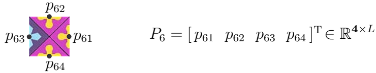
Figure 114: Demo-game piece P_6 illustrating edge-color \bullet p_{6j} \in \mathbb{R}^L counterclockwise ordering in j beginning from right.
