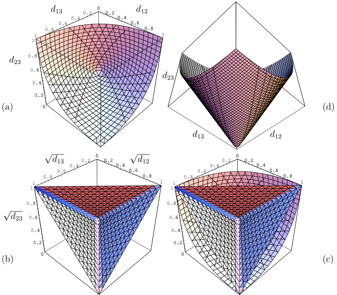
Figure 144: Relative boundary (tiled) of EDM cone \mathbb{EDM}^3 drawn truncated in isometrically isomorphic subspace \mathbb{R}^3 . (a) EDM cone drawn in usual distance-square coordinates d_{ij} . View is from interior toward origin. Unlike positive semidefinite cone, EDM cone is not selfdual; neither is it proper in ambient symmetric subspace (dual EDM cone for this example belongs to isomorphic \mathbb{R}^6 ). (b) Drawn in its natural coordinates \sqrt{d_{ij}} (absolute distance), cone remains convex ( confer §5.10); intersection of three halfspaces (1095) whose partial boundaries each contain origin. Cone geometry becomes nonconvex (nonpolyhedral) in higher dimension. (§6.3) (c) Two coordinate systems artificially superimposed. Coordinate transformation from d_{ij} to \sqrt{d_{ij}} appears a topological contraction. (d) Sitting on its vertex \mathbf{0} , pointed \mathbb{EDM}^3 is a circular cone having axis of revolution \text{dvec}(-E) = \text{dvec}(\mathbf{1}\mathbf{1}^T - I) (1128) (73). (Rounded vertex is plot artifact.)
