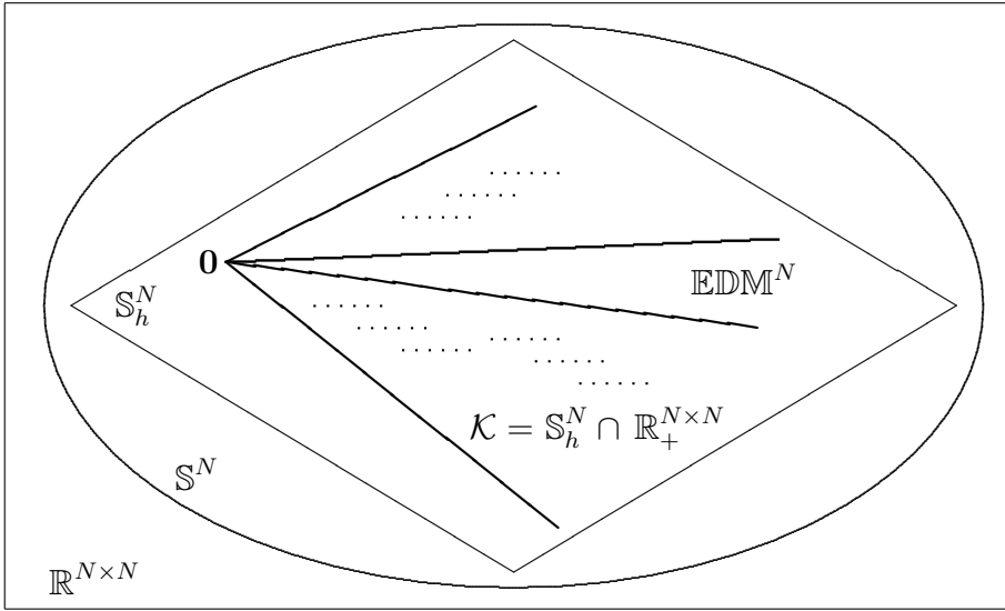
Figure 158: Pseudo-Venn diagram: The EDM cone belongs to the intersection of the symmetric hollow subspace with the nonnegative orthant; \mathbb{EDM}^N \subseteq \mathcal{K} (922). \mathbb{EDM}^N cannot exist outside \mathbb{S}_h^N , but \mathbb{R}_+^{N \times N} does.
