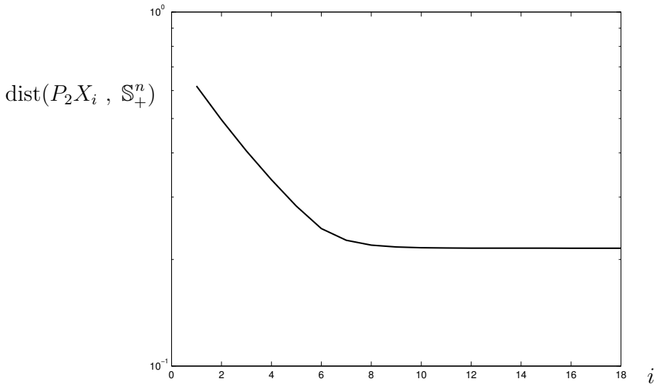
Figure 179: Distance ( confer (2121)) between positive semidefinite cone and iterate (2124) in affine subset \mathcal{A} (2117) for Laurent's completion problem; initially, decreasing geometrically.
