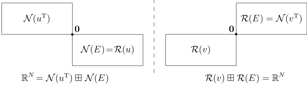
Figure 164: v^T u = 1/\zeta . The four fundamental subspaces [334, §3.6] of elementary matrix E as a linear mapping E(x) = \left(I - \frac{uv^T}{v^T u}\right)x .
