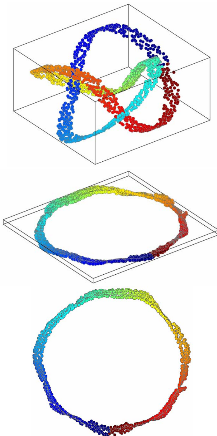
Figure 153: Trefoil ribbon ; courtesy, Kilian Weinberger. Same topological transformation algorithm with 5 nearest neighbors and N=1617 samples.
