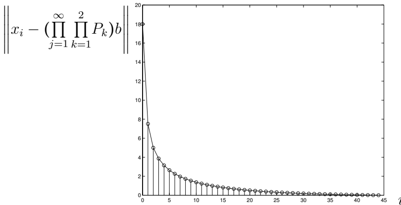
Figure 178: Example E.10.2.0.2 in \mathbb{R}^{1000} ; geometric convergence of iterates in norm.
