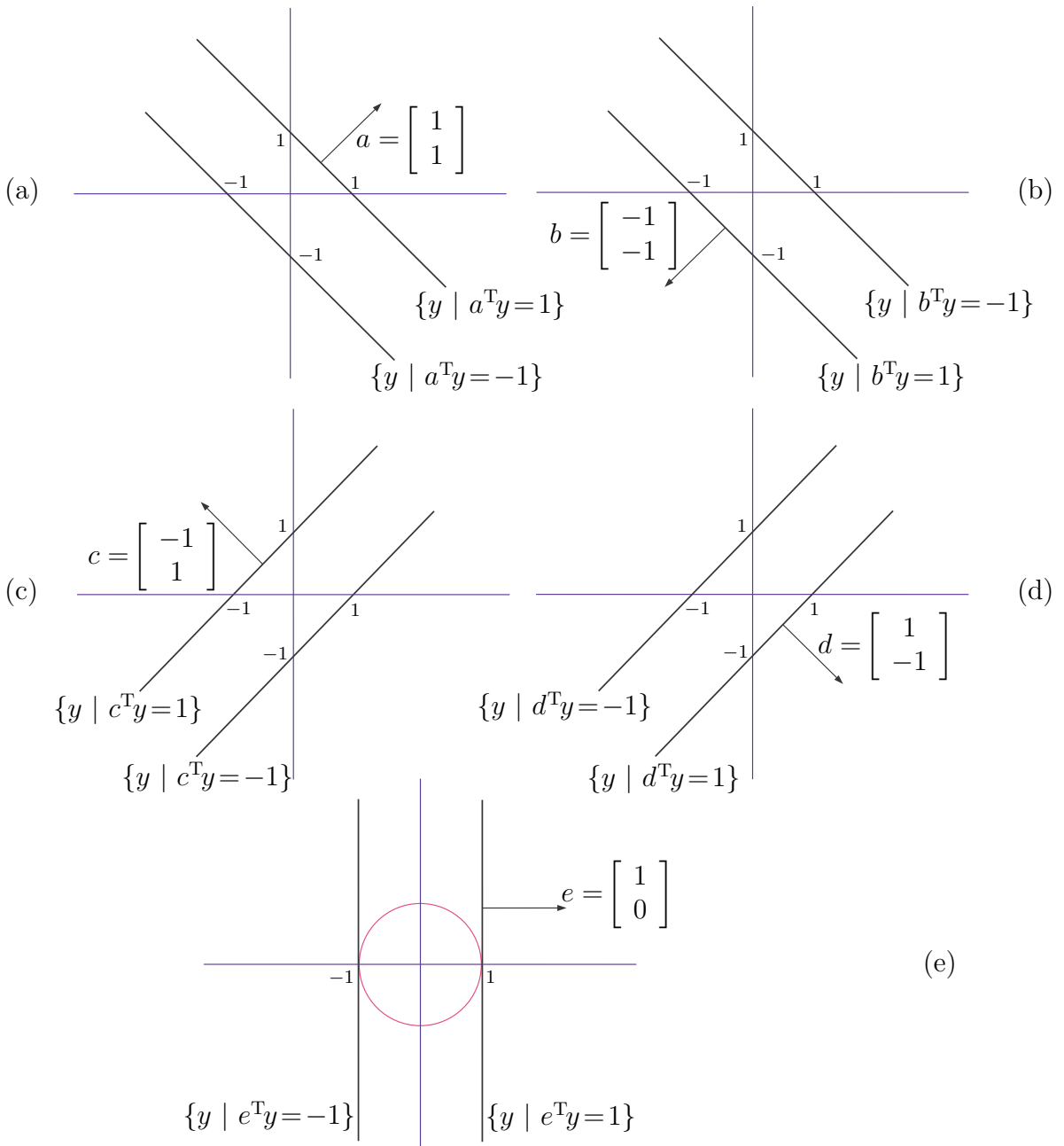
Figure 26: (a)-(d) Hyperplanes in \mathbb{R}^2 (truncated) redundantly emphasize: hyperplane movement opposite to its normal direction minimizes vector inner-product. This concept is exploited to attain analytical solution of linear programs by visual inspection; e.g. , Example 2.4.2.6.2, Exercise 2.5.1.2.2, Example 3.4.0.0.2, [61, exer.4.8-exer.4.20]. Each graph is also interpretable as contour plot of a real affine function of two variables as in Figure 73. (e) |\beta|/\|\alpha\| from \partial\mathcal{H} = \{x \mid \alpha^T x = \beta\} represents radius of hypersphere about \mathbf{0} supported by any hyperplane with same ratio |\text{inner product}|/\text{norm} .
