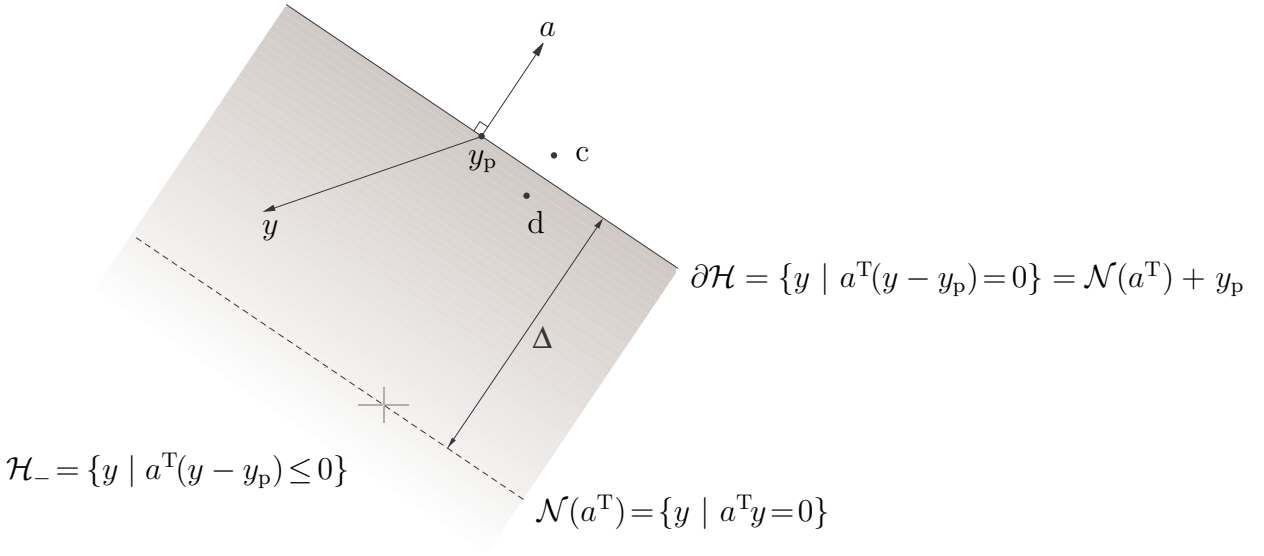
Figure 25: Hyperplane illustrated \partial\mathcal{H} is a line partially bounding halfspaces \mathcal{H}_- and \mathcal{H}_+ in \mathbb{R}^2 . Shaded is a rectangular piece of semiinfinite \mathcal{H}_- with respect to which vector a is outward-normal to bounding hyperplane; vector a is inward-normal with respect to \mathcal{H}_+ . Halfspace \mathcal{H}_- contains nullspace \mathcal{N}(a^T) (dashed line through origin) because a^T y_p > 0 . Hyperplane, halfspace, and nullspace are each drawn truncated. Points c and d are equidistant from hyperplane, and vector c - d is normal to it. \Delta is distance from origin to hyperplane.
