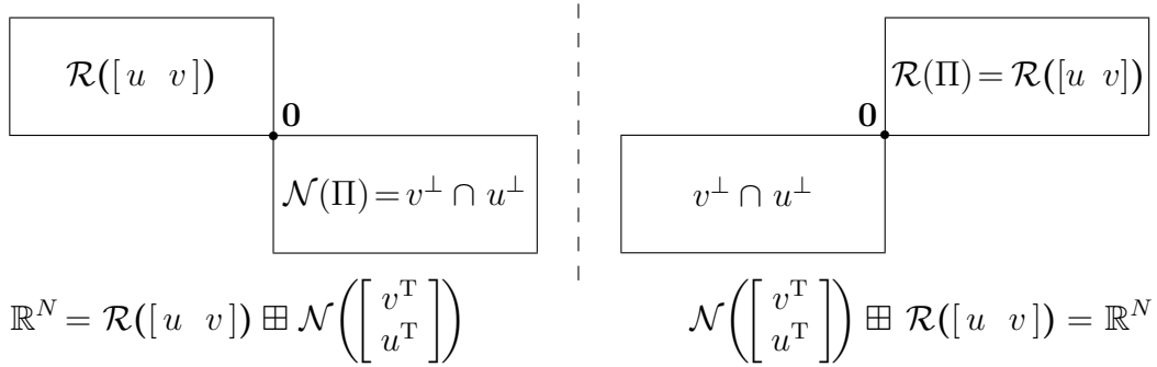
Figure 163: The four fundamental subspaces [334, §3.6] of a doublet \Pi = uv^T + vu^T \in \mathbb{S}^N . \Pi(x) = (uv^T + vu^T)x is a linear bijective mapping from \mathcal{R}([u \ v]) to \mathcal{R}([u \ v]) .
