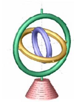
Figure 165: Gimbal : a mechanism imparting three degrees of dimensional freedom to a Euclidean body suspended at the device's center. Each ring is free to rotate about one axis. (Courtesy of The MathWorks Inc.)
