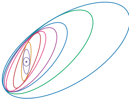
Figure 132: Some fitted contours of equal signal power in \mathbb{R}^2 transmitted from a commercial cellular telephone • over about 1 mile suburban terrain outside San Francisco in 2005. Data courtesy Polaris Wireless. [323]
