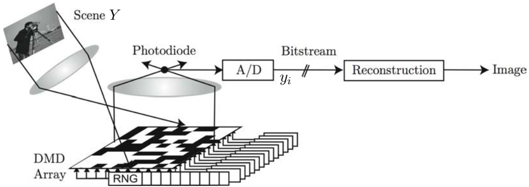
Figure 119: One-pixel camera. [346] [372] Compressive imaging camera block diagram. Incident lightfield (corresponding to the desired image Y ) is reflected off a digital micromirror device (DMD) array whose mirror orientations are modulated in the pseudorandom pattern supplied by the random number generators (RNG). Each different mirror pattern produces a voltage at the single photodiode that corresponds to one measurement y_i .
